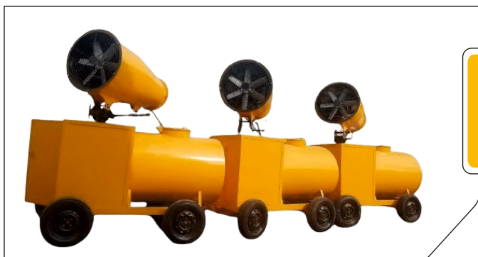
Anti Smog Gun Electric Trolley / Truck Mounted Throw upto 35 mtrs Water Tank - 1000 to 1500 ltrs. Tilting Angle- 12 - 55 Degree Horiz. Rotation - 350 Degree
